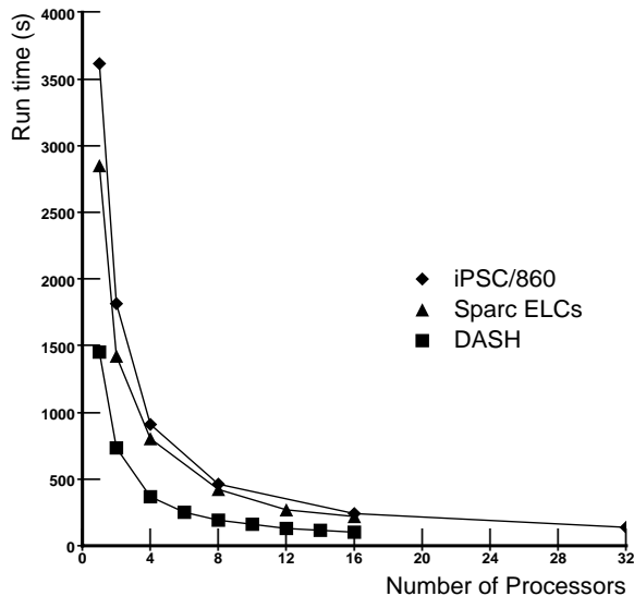
Figure 8: Running Times for Liquid Water Simulation
