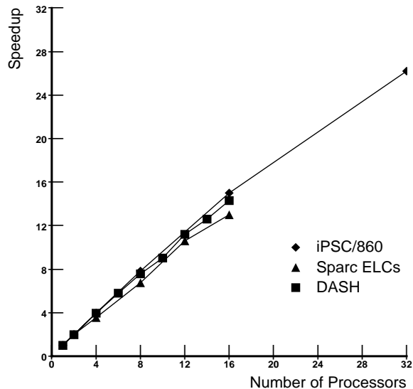
Figure 9: Speedups for Liquid Water Simulation
